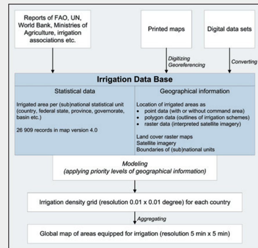
Fig. 4: Scheme of mapping methodology
