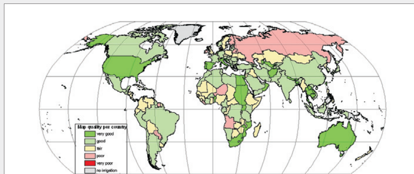
Fig. 5: Global Map of Irrigation Areas version 4 - map quality at the country scale
