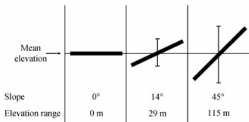
Fig. 7. Effect of raster cell inclination (slope) on the elevation range spanned in one raster cell. The elevation ranges given apply to the directions NE, SE, SW and NW. For the cardinal directions, they are 0 m, 20 m and 81 m, respectively.
