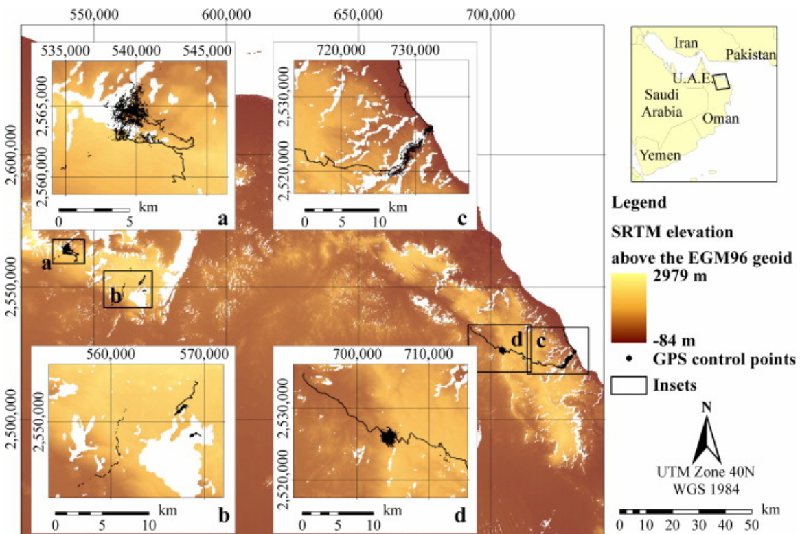
Fig. 2. Location of the GPS control points in the Oman Mountains. The insets a–d show the surroundings of the oases, where most of the positions were recorded. The small map in the upper right corner shows the location of the large map window on the Arabian Peninsula.
