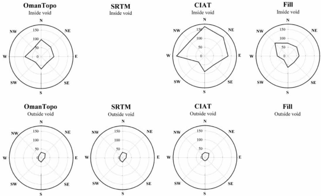
Fig. 6. Standard deviations of the \Delta GPS values derived from the four surfaces, inside and outside the void areas in the SRTM model, according to the bearing of the slope at the GPS location.
