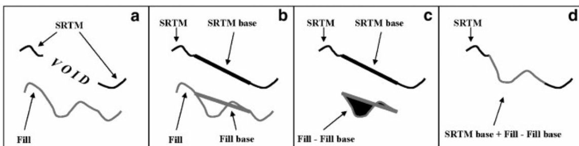
Fig. 3. Illustration of the process used to merge the two elevation surfaces. For the void area in the SRTM model and for the corresponding region in the fill surface (a), TINs are calculated from points at the edges to create base surfaces (b). The fill base surface is then subtracted from the fill surface (c) and added on top of the SRTM base surface (d) to obtain a seamless DEM.
