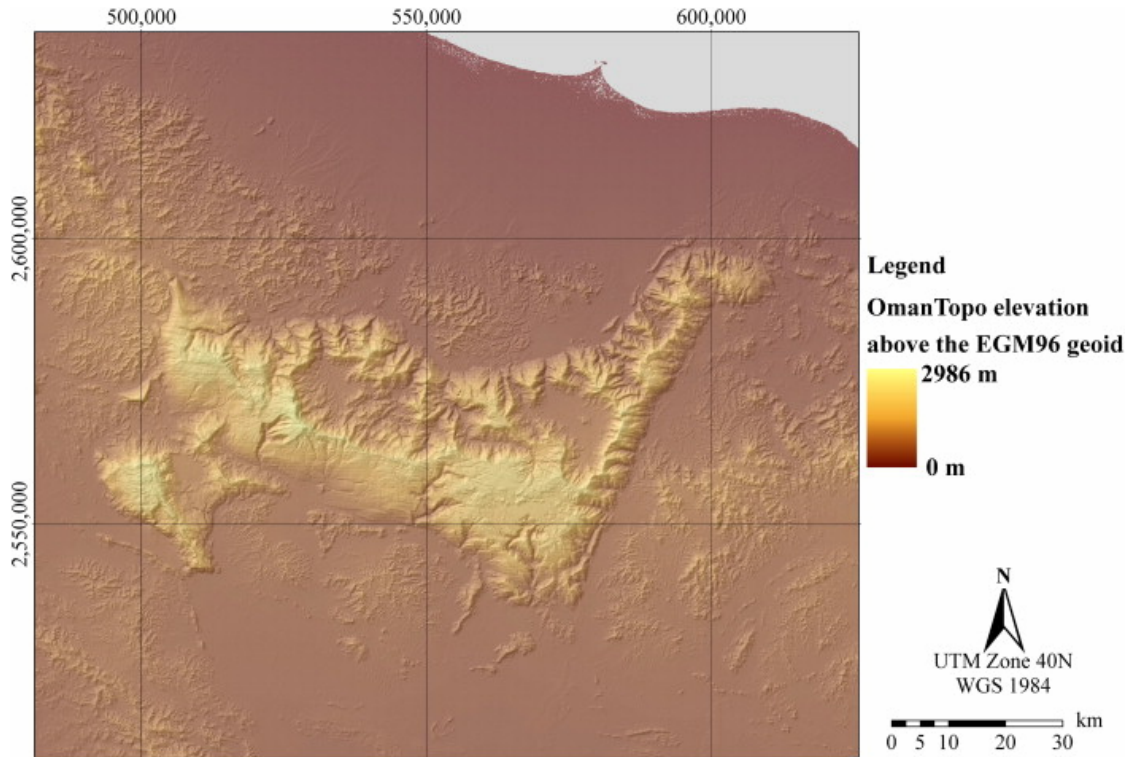
Fig. 5. Shaded relief of OmanTopo for visual inspection.
